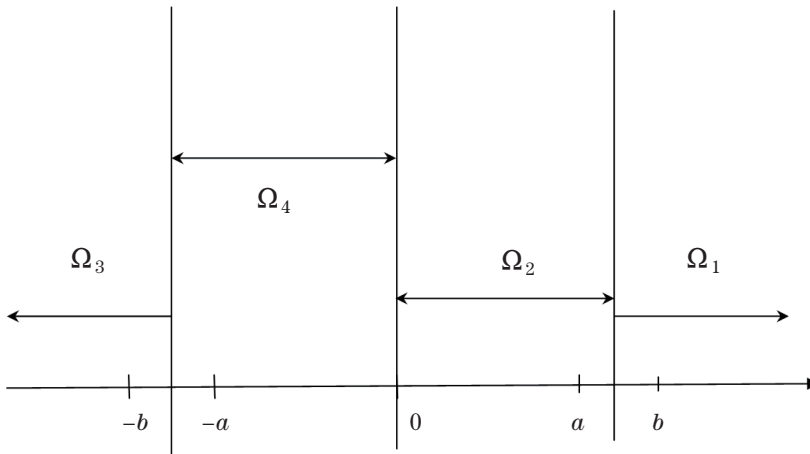
Figure 4 The domains \Omega_1, \dots, \Omega_4 .
